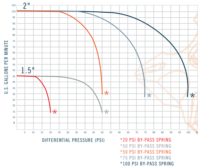
PUMP CURVE DATA
